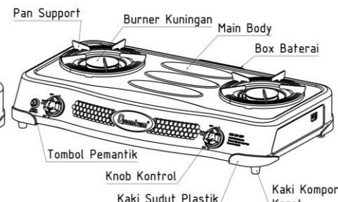
MODEL TYPE: QGC-201 DEP
